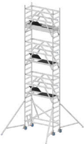
RS4S075x185x600
