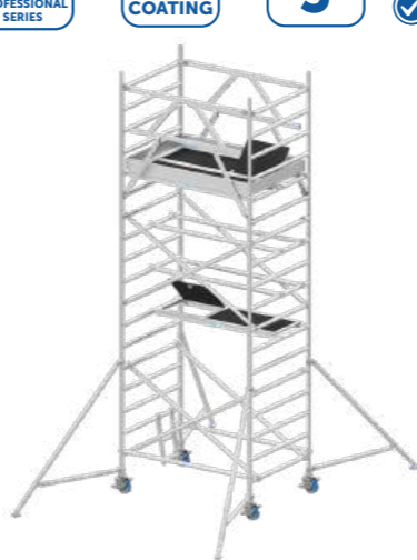
RS135x185x400
