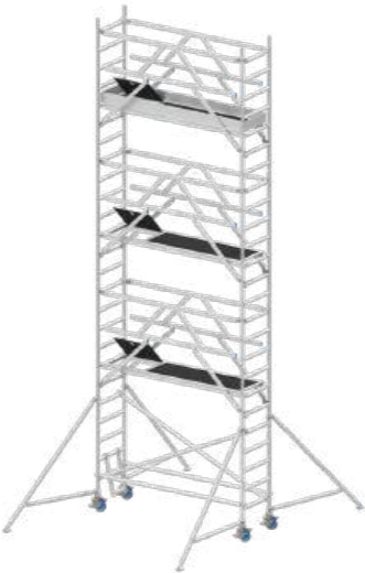
RS4S075x245x600
