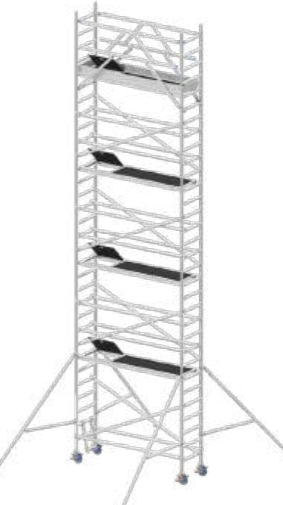
RS075x245x800
